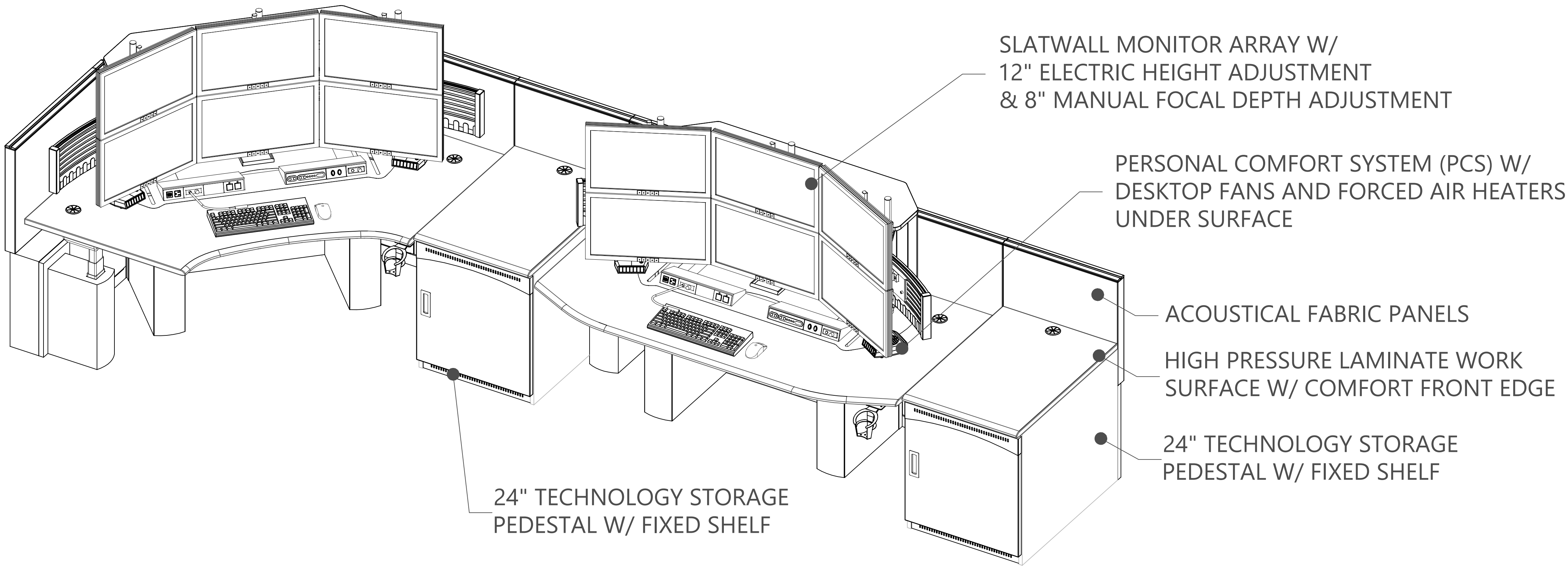
PERSPECTIVE VIEW
