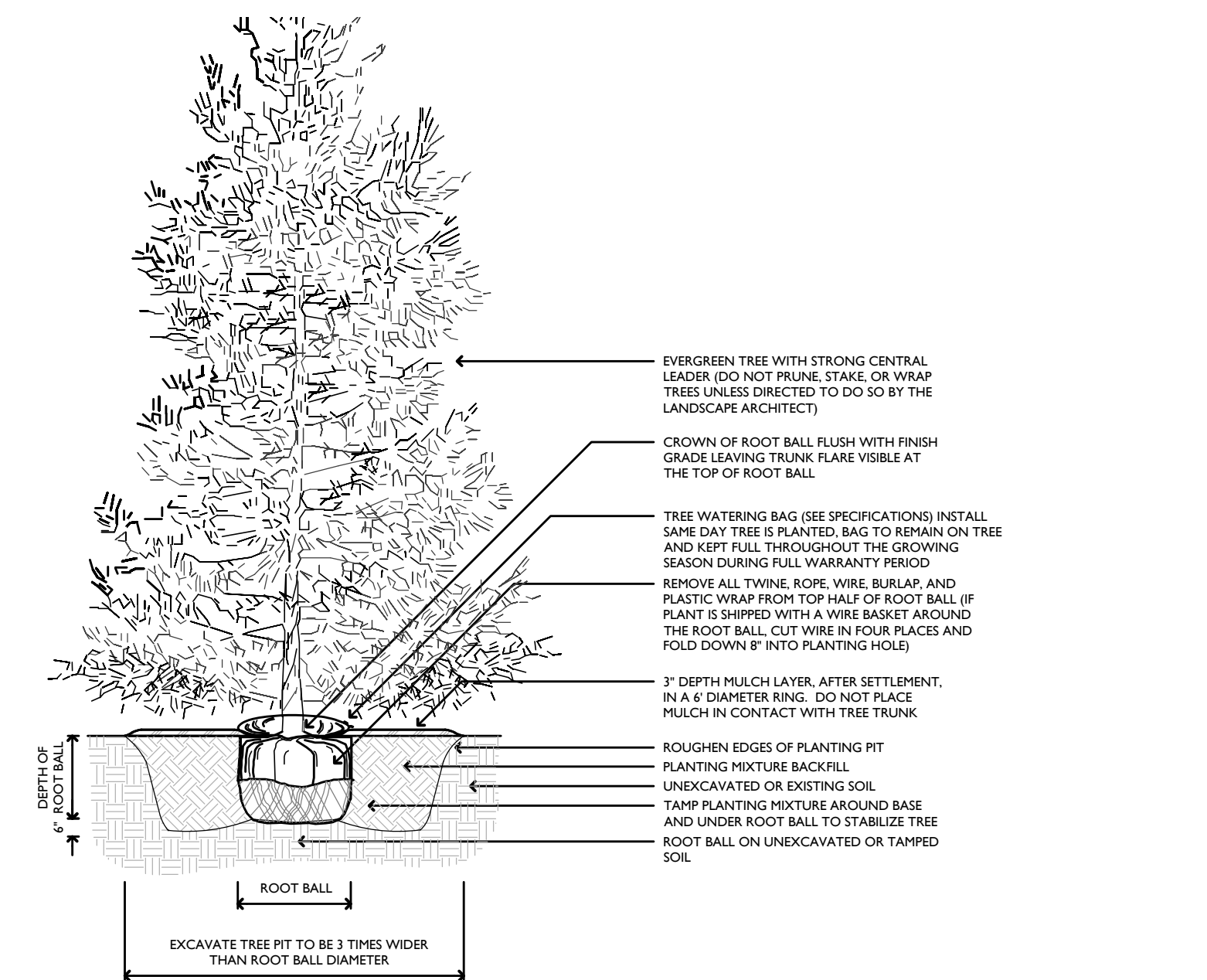
6 EVERGREEN TREE INSTALLATION DETAIL SCALE: 1/4" = 1'-0"
