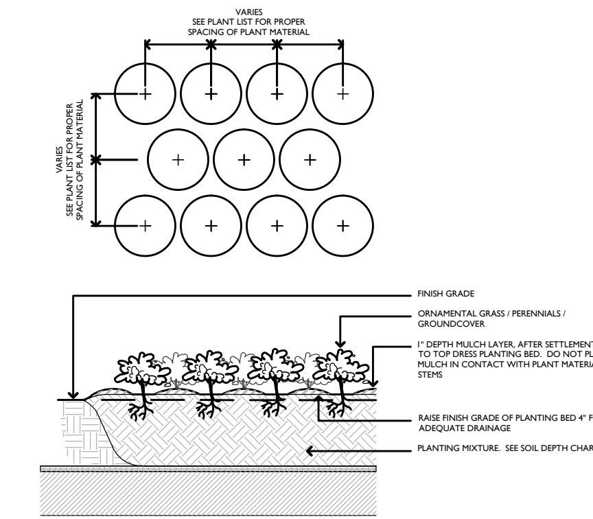
3 ORNAMENTAL GRASS, PERENNIAL AND GROUNDCOVER INSTALLATION DETAIL NOT TO SCALE
