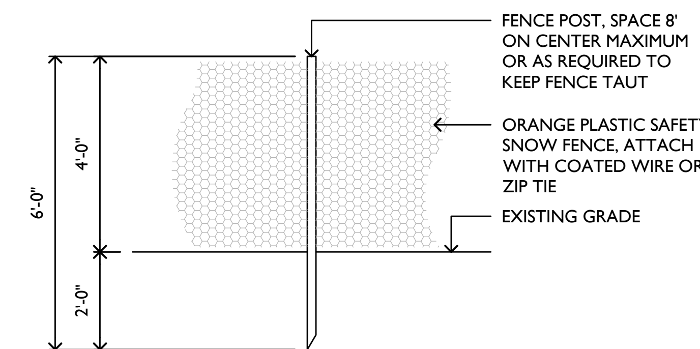
3 TREE PROTECTION FENCE DETAIL SCALE: NOT TO SCALE
