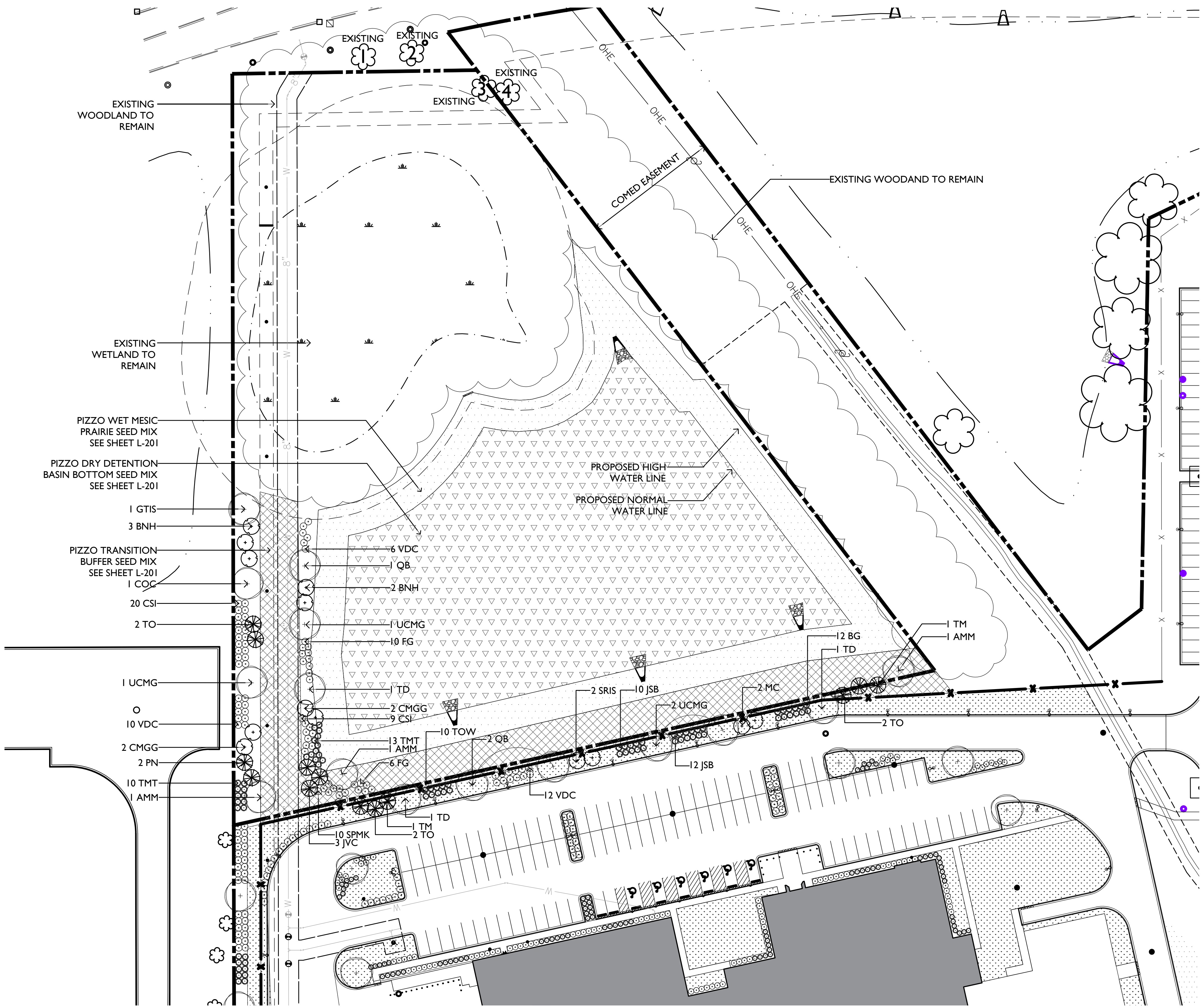
3 LANDSCAPE PLAN - WETLAND NORTH SCALE: 1" = 40'-0"
