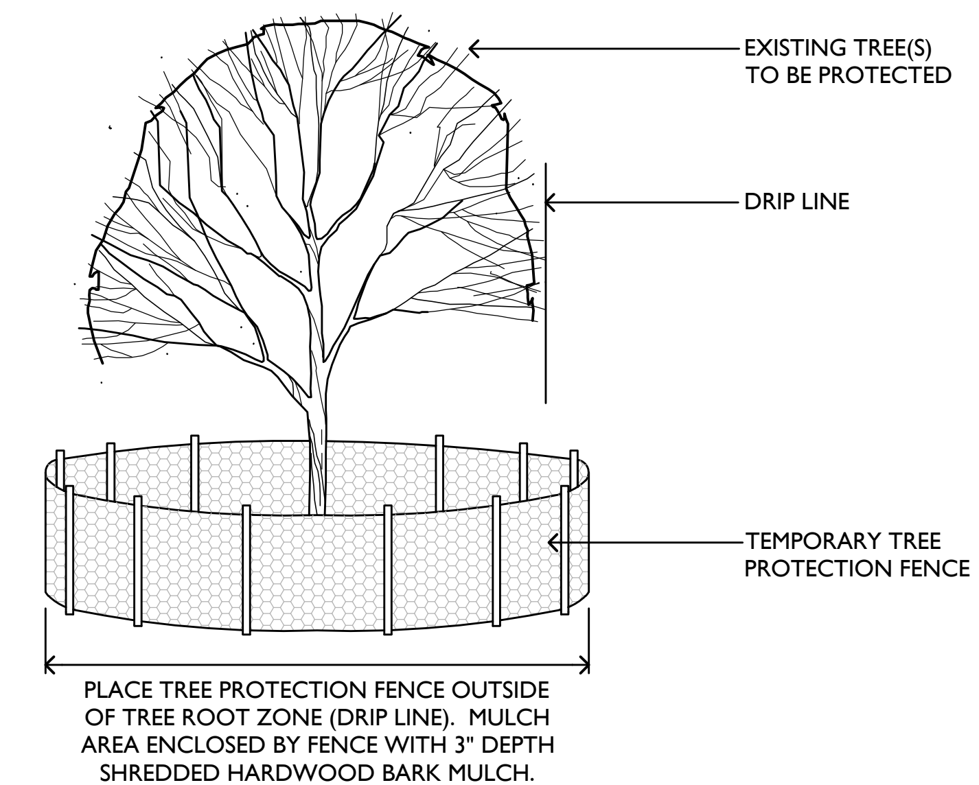
2 TREE PROTECTION FENCE DETAIL SCALE: NOT TO SCALE
