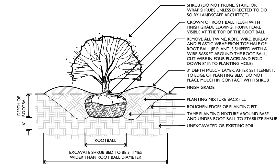
2 SHRUB INSTALLATION DETAIL NOT TO SCALE
