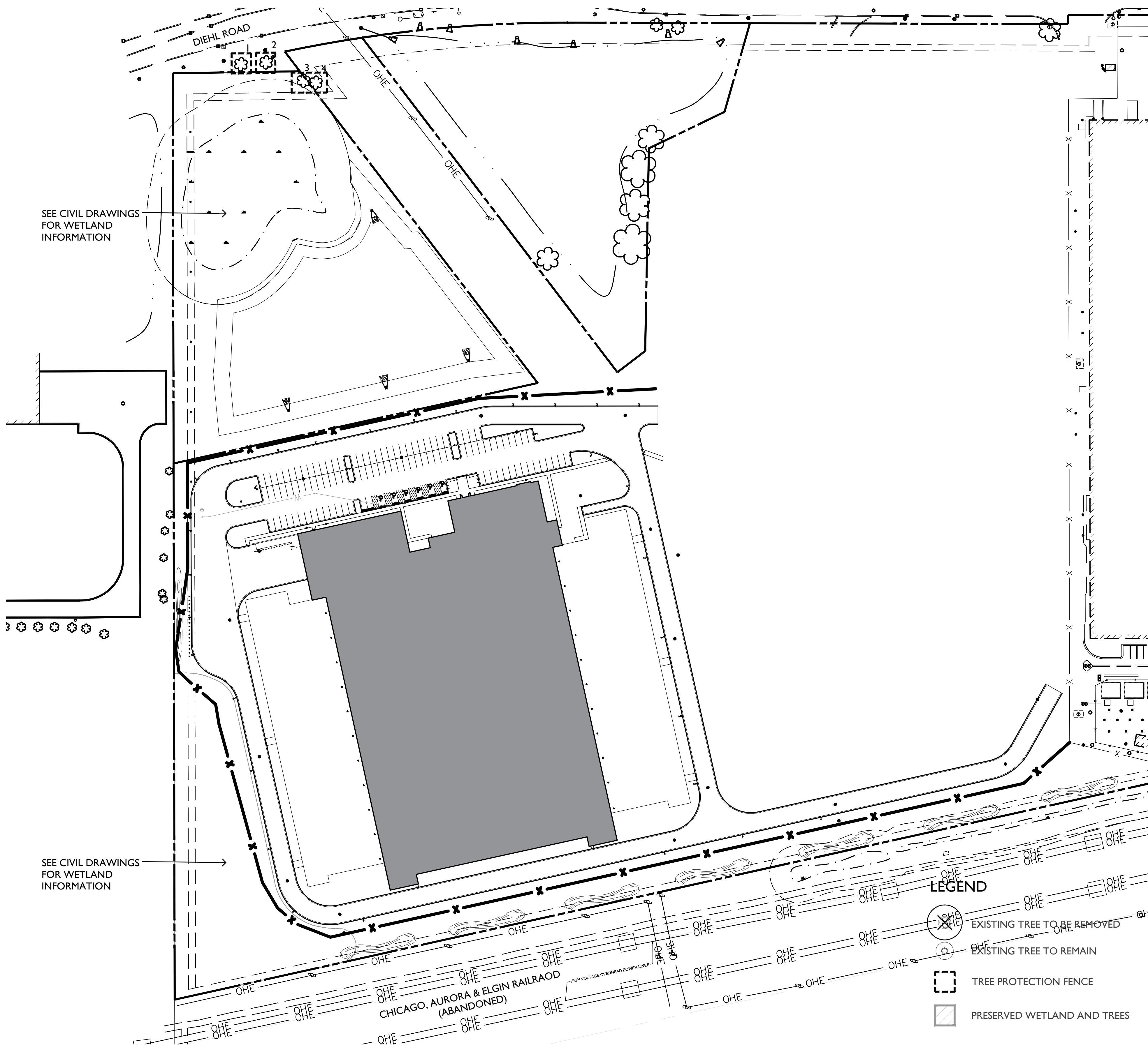
2 TREE PRESERVATION AND REMOVAL PLAN SCALE: 1" = 80'-0"
