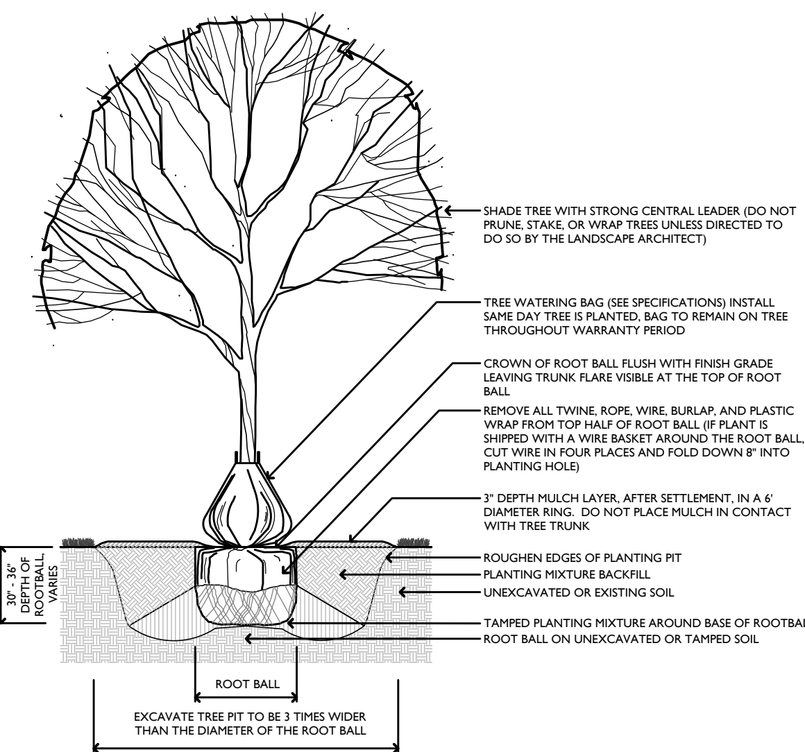
4 DECIDUOUS TREE INSTALLATION DETAIL SCALE: 1/4" = 1'-0"
