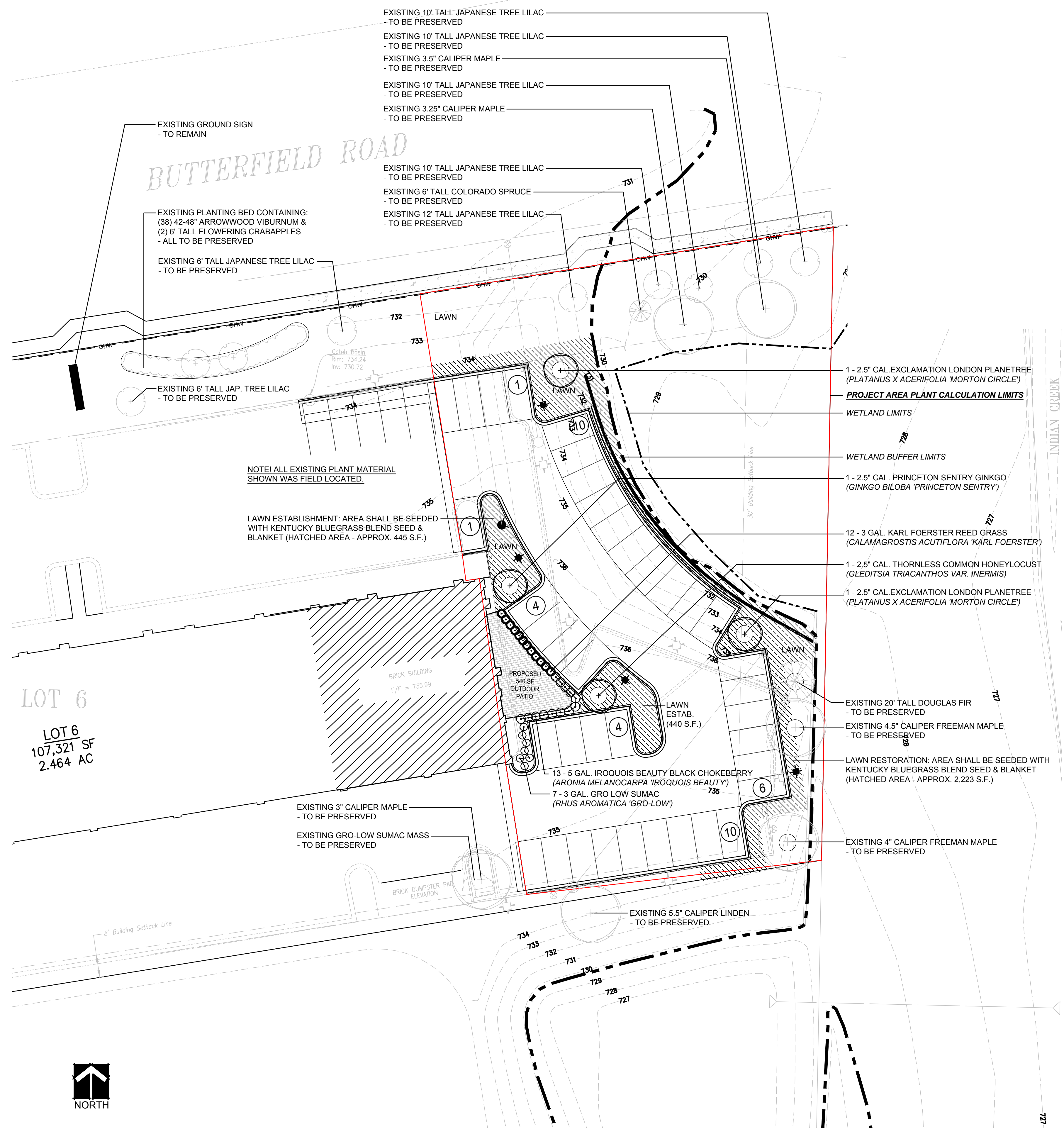
LANDSCAPE PLAN - PROPOSED CONDITIONS SCALE: 1" = 20'-0"
