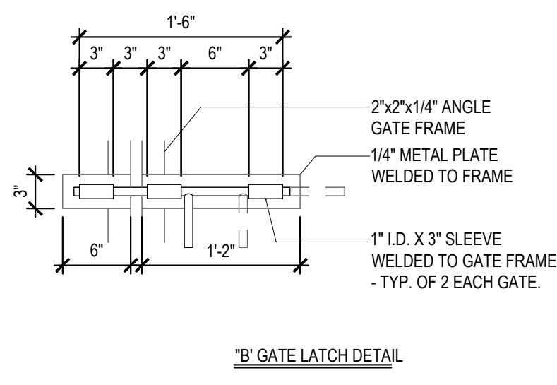
DUMPSTER GATE LATCH DETAILS 15
