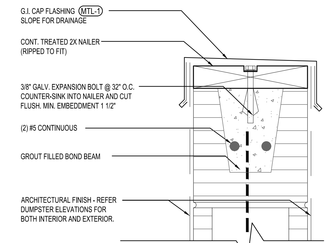
DUMPSTER CAP DETAIL 17
