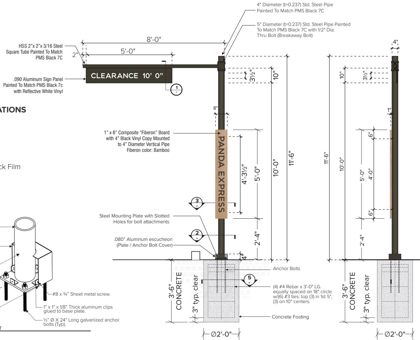
SIDE VIEW - NON-ILLUMINATED CLEARANCE BAR SCALE: 1:40
