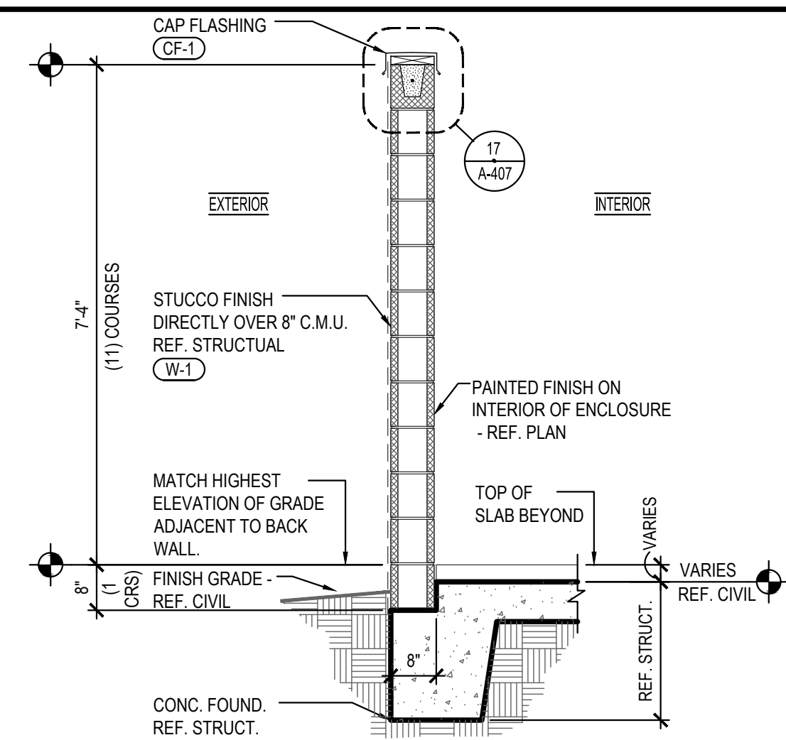
TRASH ENCLOSURE WALL SECTION 08
