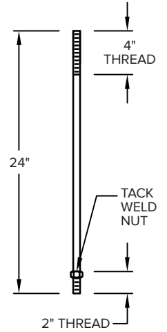
ANCHOR BOLT DETAIL Ø5/8" 18-8 STAINLESS STEEL
