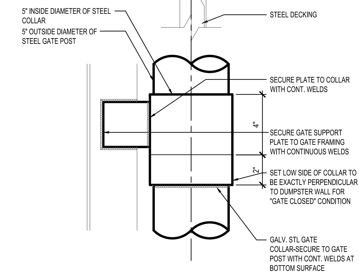
HINGE DETAIL 13
