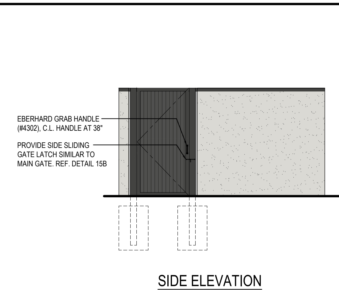
SIDE ELEVATION 04
