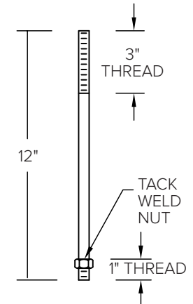
ANCHOR BOLT DETAIL Ø3/8" 18-8 STAINLESS STEEL
