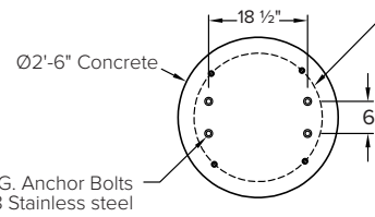
PLAN VIEW QTY. CONCRETE: 1.0 CU. YDS. FOOTING DETAIL nts
