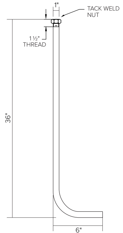
ANCHOR BOLT DETAIL (NTS) Ø1" ASTM F-1554 GR. 36 STEEL
