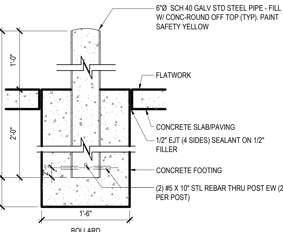
BOLLARD AT DUMPSTERS 10
