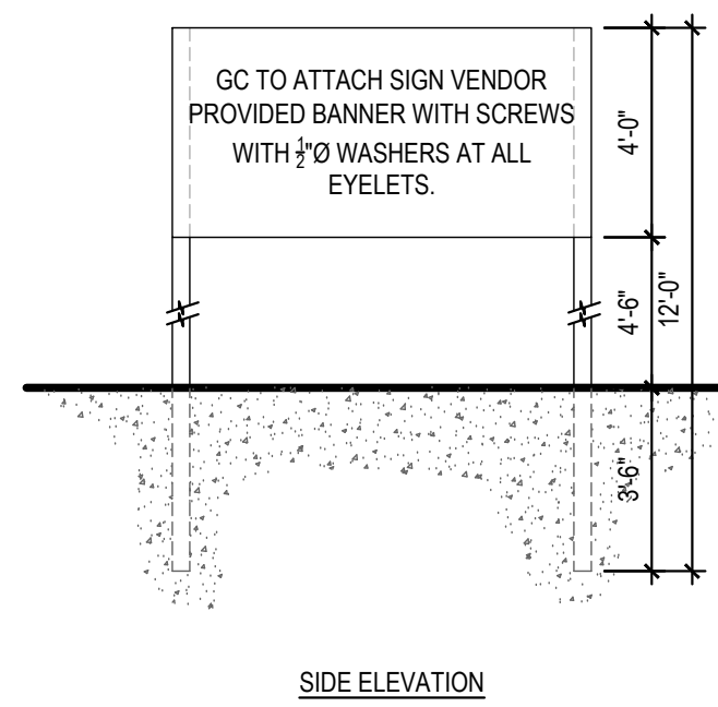
"COMING SOON" SIGN DETAIL 16
