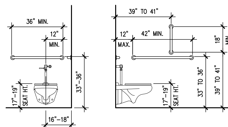
WATER CLOSET AND GRAB BAR MOUNTING LOCATIONS
