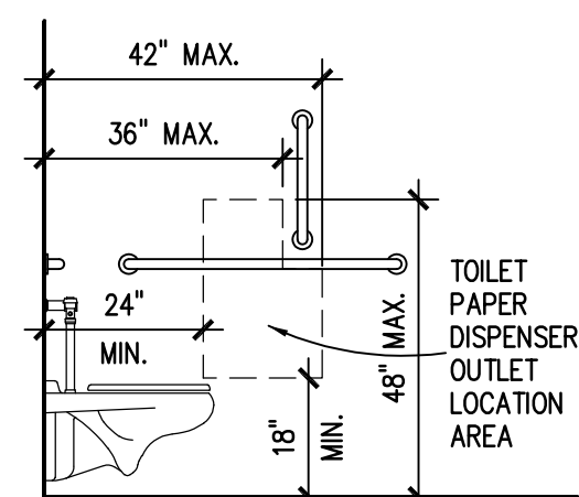
ICC A117.1 REQUIREMENTS (RECESSED DISPENSERS)
