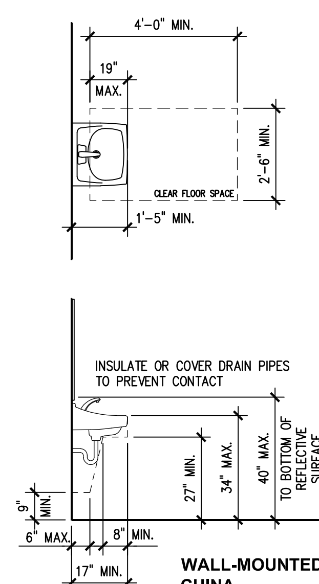
WALL-MOUNTED CHINA
