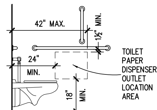
ICC A117.1 REQUIREMENTS (PROTRUDING DISPENSERS)
