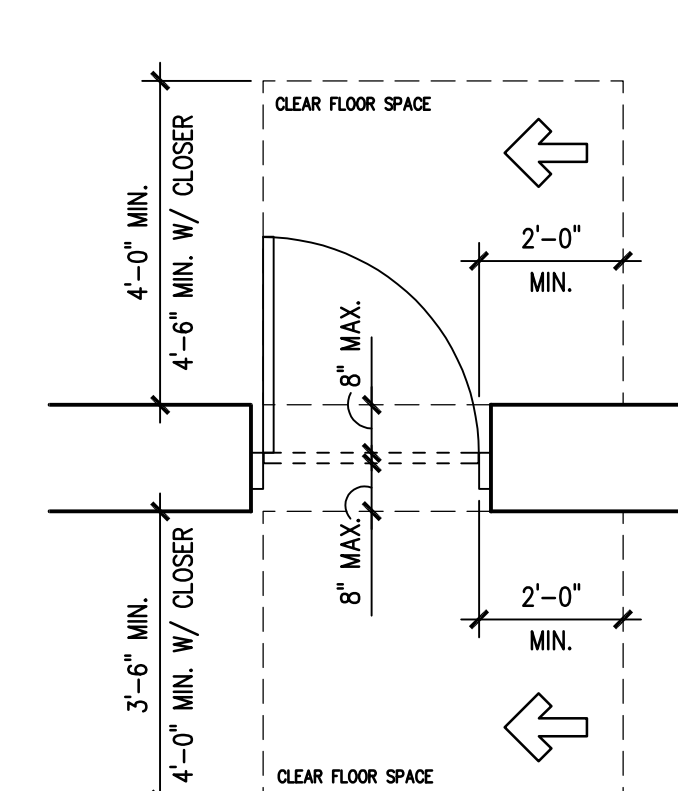
SIDE-SWINGING DOORS
