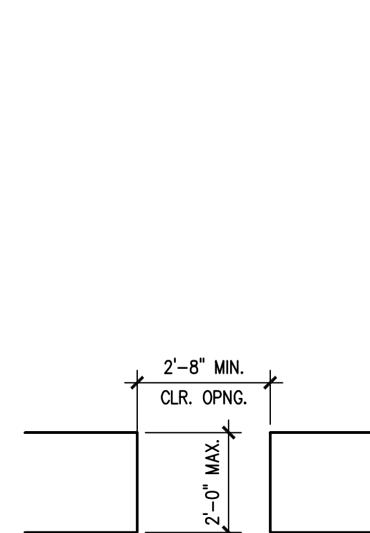
OPENINGS WITHOUT DOORS
