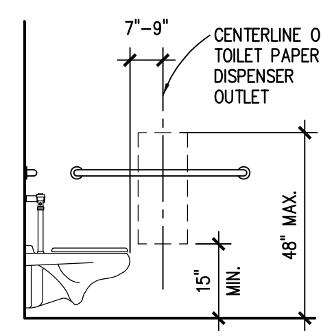
ILLINOIS ACCESSIBILITY CODE REQUIREMENTS (ALL DISPENSERS)
