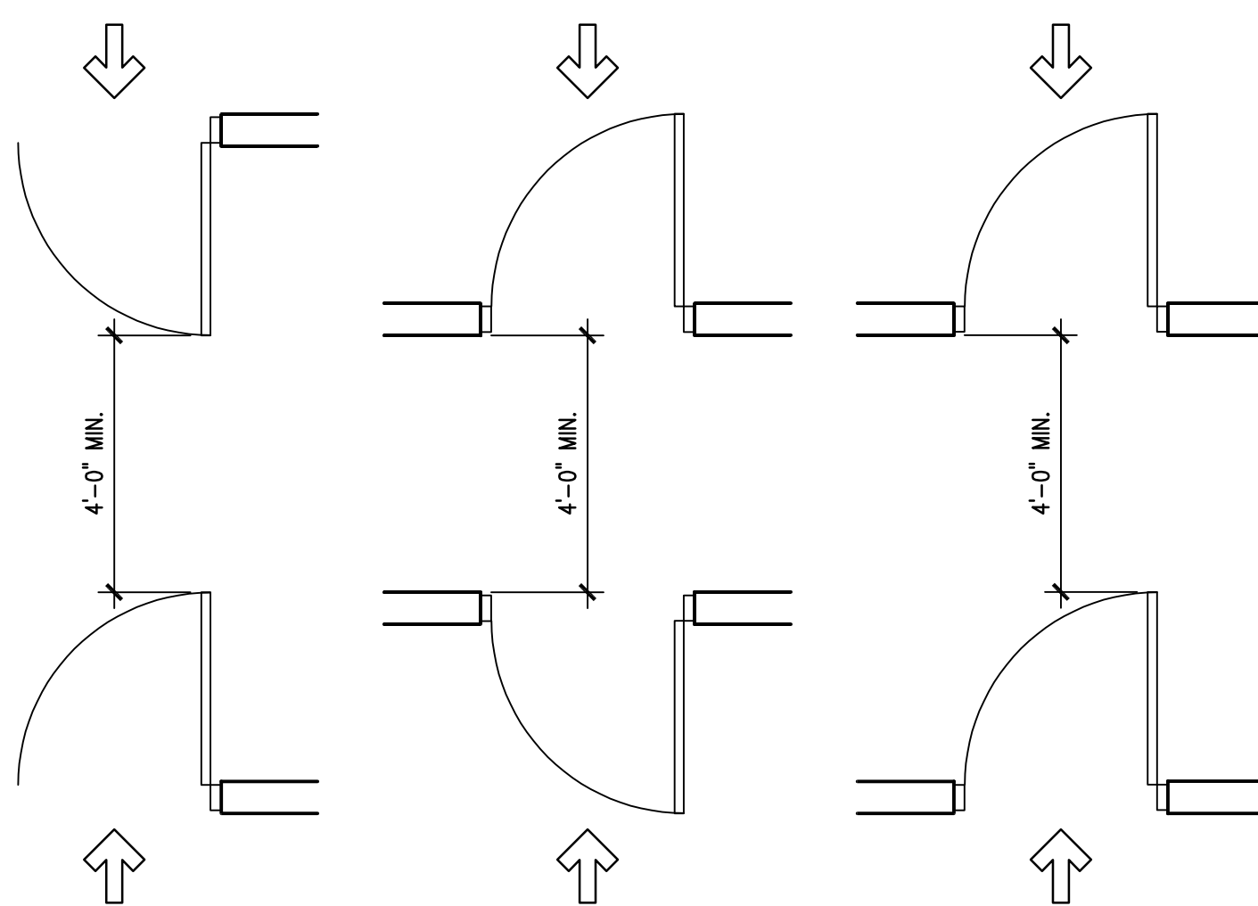
DOORS IN SERIES
