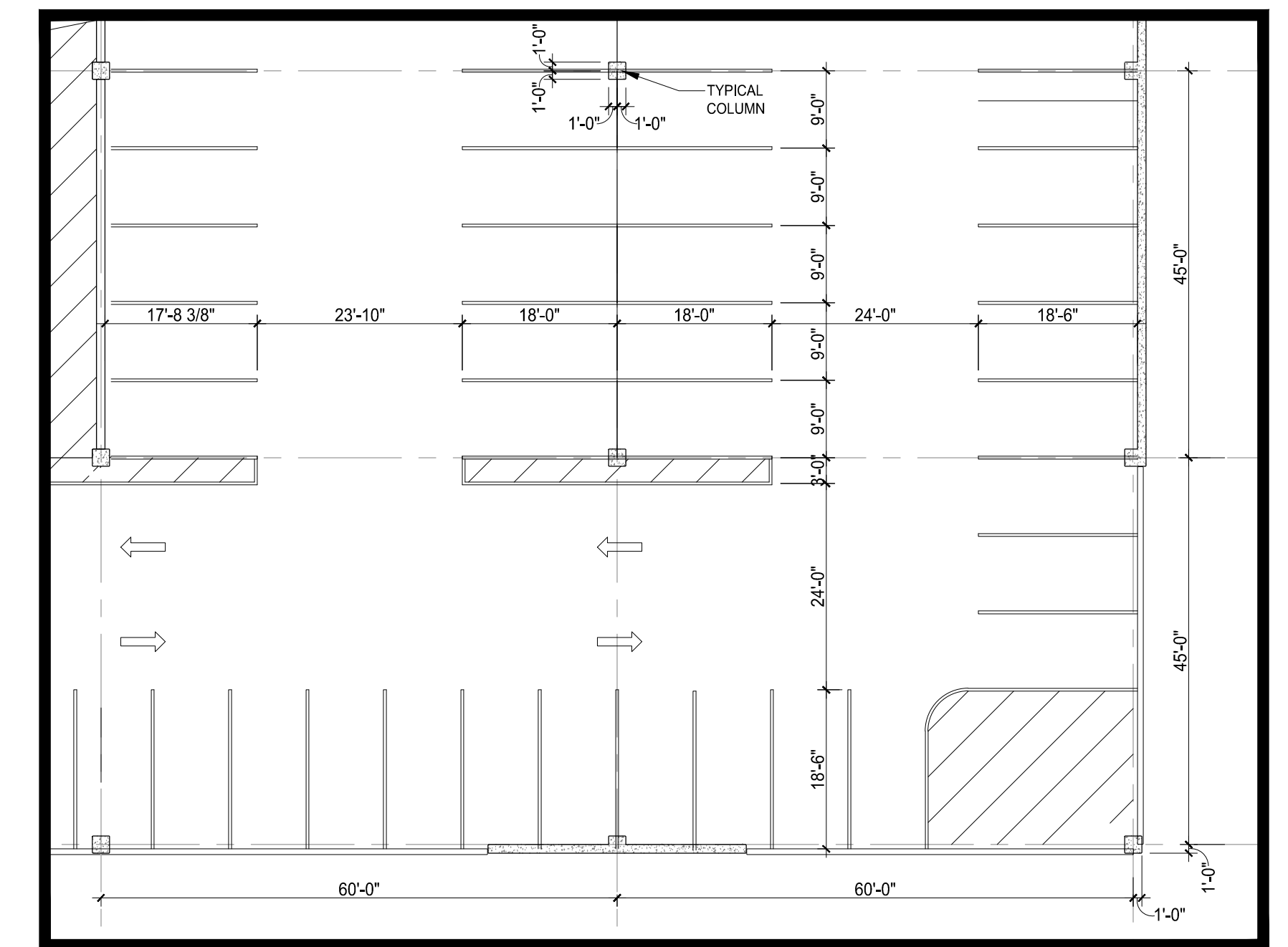
TYPICAL PARKING & DRIVE AISLE DIMENSIONS SCALE: 1/16" = 1'-0"
