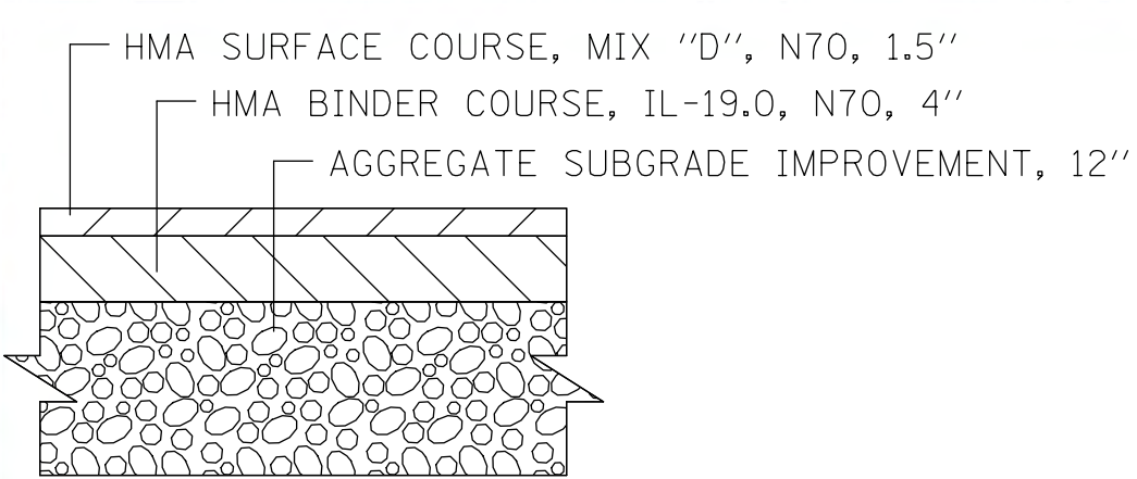
FULL DEPTH HMA PAVEMENT
