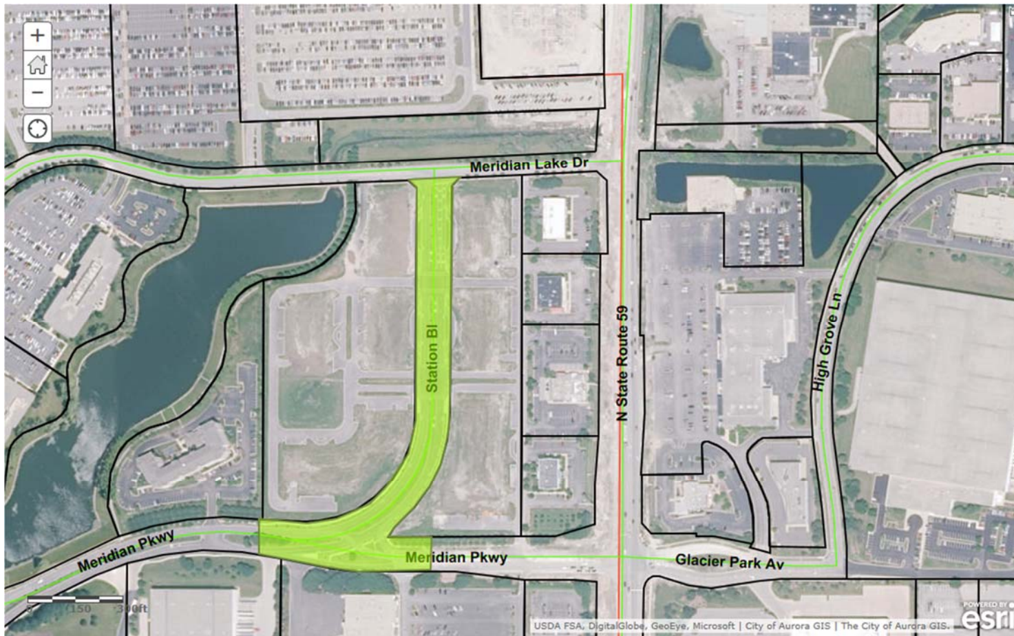
Metro 59 – Station Blvd. Roadway Improvements – COA Case No. 11.399
