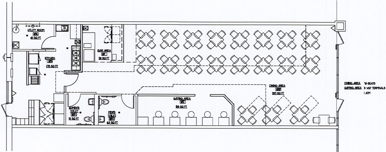
FLOOR SEATING PLAN SCALE: 1/4" = 1'-0"
