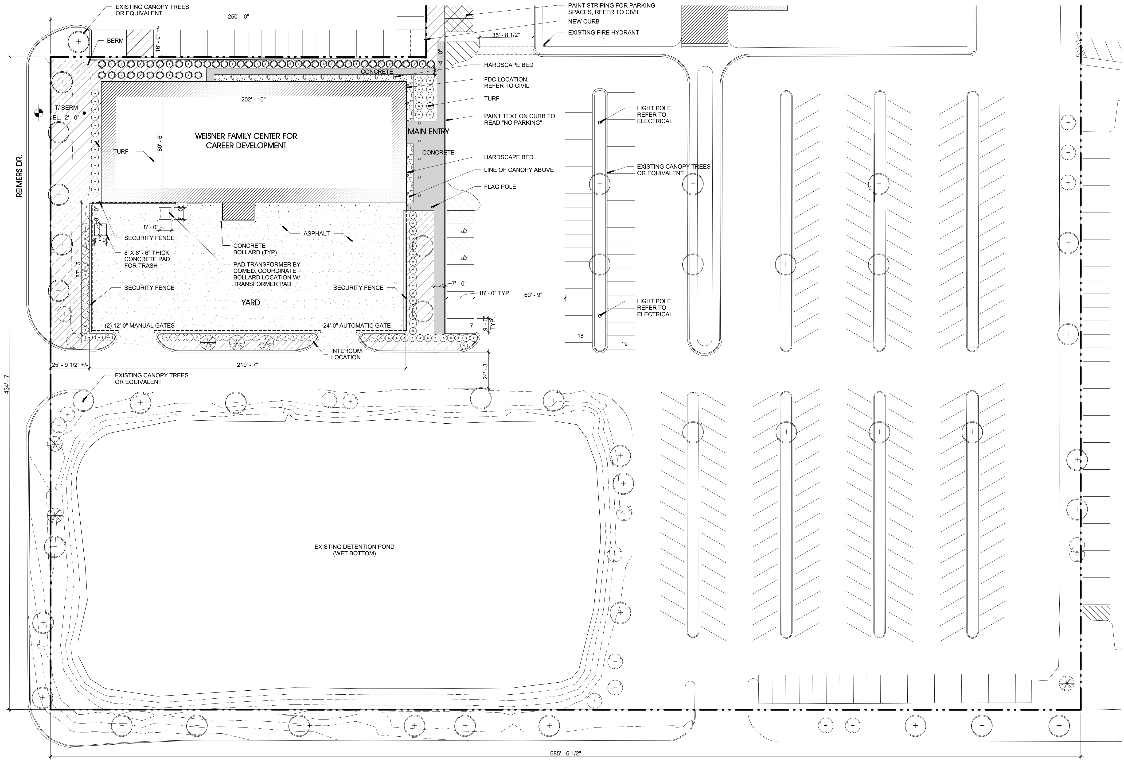
NORTH 1 LANDSCAPE PLAN 1" = 30'-0"
