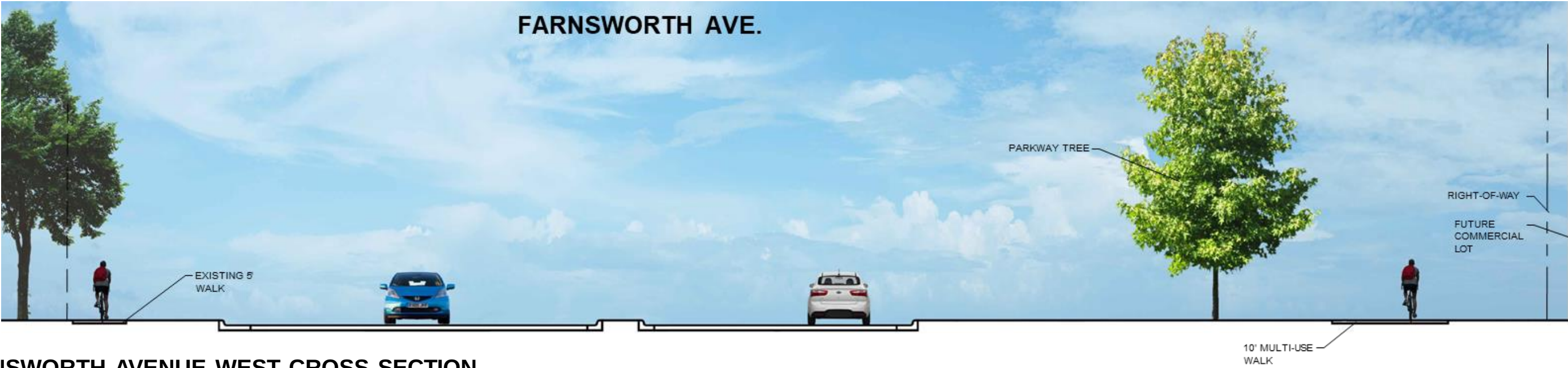
FARNSWORTH AVENUE WEST CROSS SECTION
