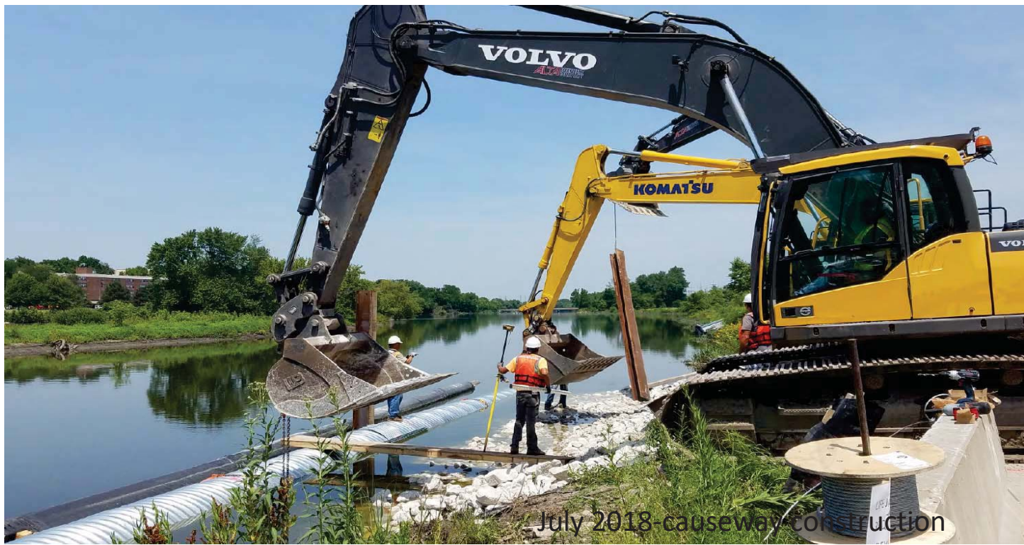
July 2018 causeway construction
